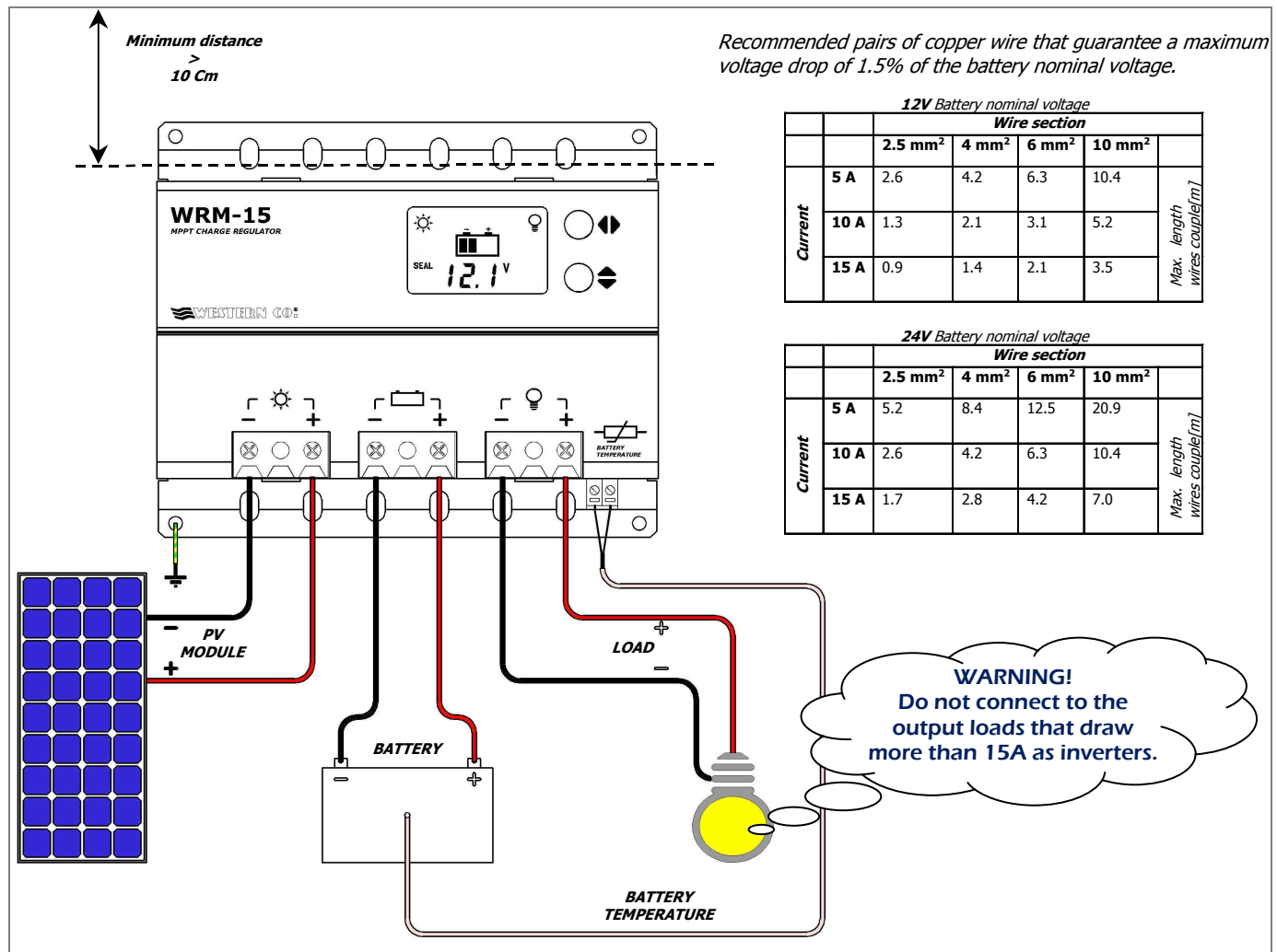
Fig. 2 Connection scheme
